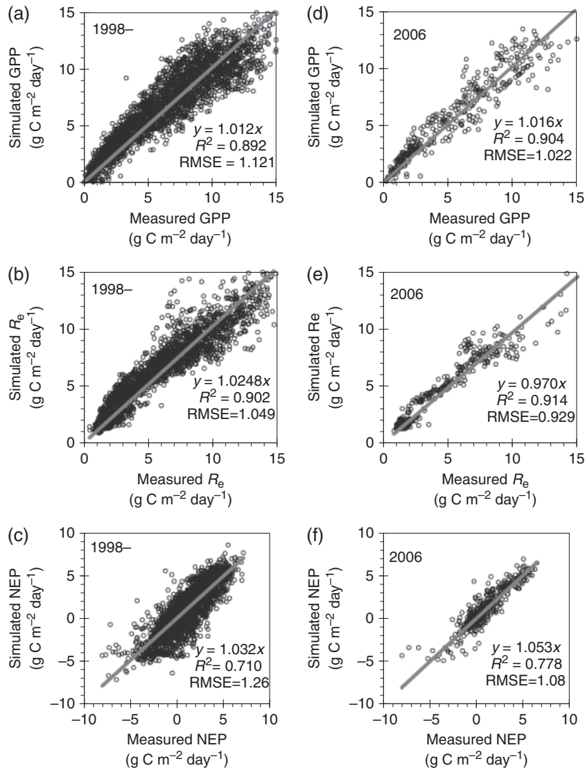
Fig. 4 Comparison of BEPS predicted and EC tower measured daily gross primary productivity (GPP), ecosystem respiration ( R_e ) and net ecosystem productivity (NEP) at DF49 for nonfertilized years, (a)–(c) for the EnKF applied years 1998–2005, and (d)–(f) for the validation year 2006. BEPS, Boreal Ecosystem Productivity Simulator; RMSE, root mean square error.
