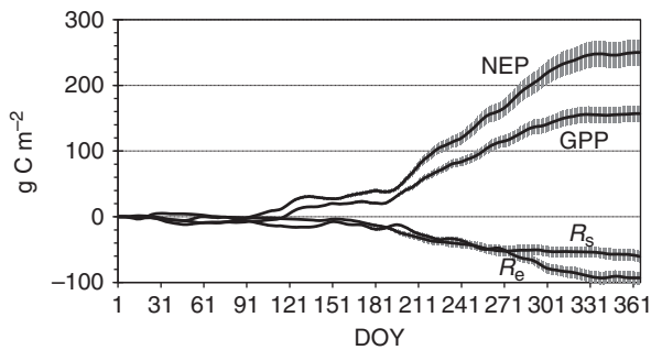
Fig. 10 Cumulative N fertilization effects on C component fluxes with \pm 1 SE in 2007 at DF49, which were estimated as the differences between the measured C fluxes and the corresponding modeled values. Standard errors were estimated using the \pm 1 SD of optimized model parameters. The C component fluxes are gross primary productivity (GPP), ecosystem respiration ( R_e ), soil respiration ( R_s ), and net ecosystem respiration (NEP).
