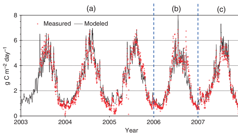
Fig. 5 BEPS predicted and measured daily soil respiration ( R_s ) using an auto-chamber at DF49 (a) for the EnKF applied years 2003–2005, (b) for the model validation year 2006, and (c) for the first-postfertilization year 2007. BEPS, Boreal Ecosystem Productivity Simulator; EnKF, ensemble Kalman filter.
